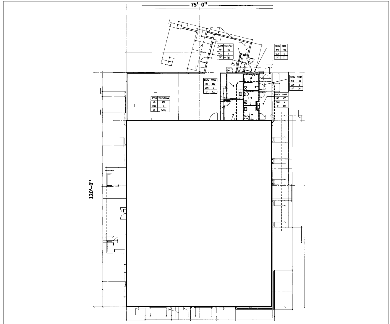
04 – Floorplan
